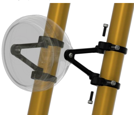
Mounting example for the lamp holder 1, 2, 3
